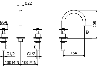
art. P1-BD50 3 holes deck mounted basin mixer
