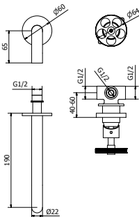
art. P1-BW02 Wall mounted basin mixer - 2 pcs
