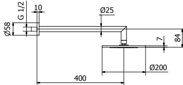
art. P1-KS02 Shower arm and round shower head Ø200mm
