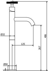
art. P1-BD01 Medium wash basin mixer short spout art. P1-KE01 Extension kit
