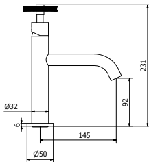
art. P1-BD02 Medium wash basin mixer long spout
