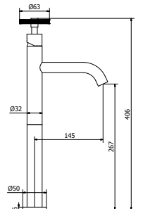
art. P1-BD02 Medium wash basin mixer long spout art. P1-KE01 - .. Extension kit
