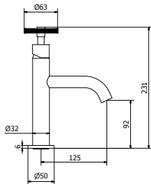
art. P1-BD01 Medium wash basin mixer short spout
